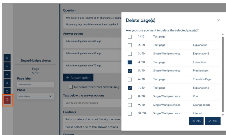
Figure 21 Page deletion.
